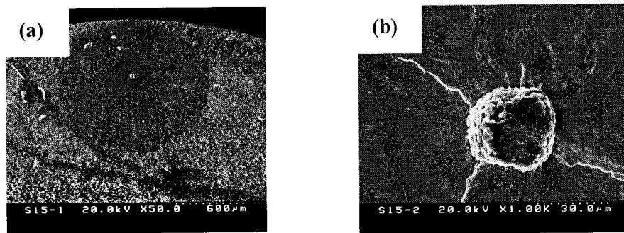
Fig. 9 SEM micrographs of interior-originating fracture after the UCFT; (a) lower magnification view of fish-eye crack and (b) enlargement of fish-eye
