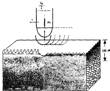
Fig. 1 Process of the UCFT
