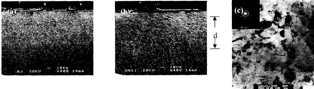
Fig.3 Microstructure of SKD 61; (a) before and (b) after the UCFT (c) UCFT treated surface layers observed by TEM
