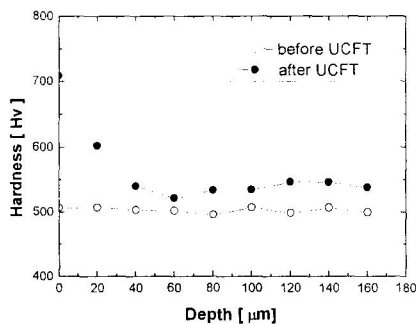
Fig.4 Variation of micro Vickers hardness residual stress for before and after by the UCFT
