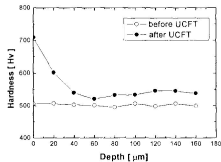
Fig. 5 Variation of compressive and depth by the UCFT
