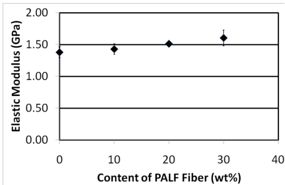
Figure 7. Elastic modulus as a function of PALF fiber
