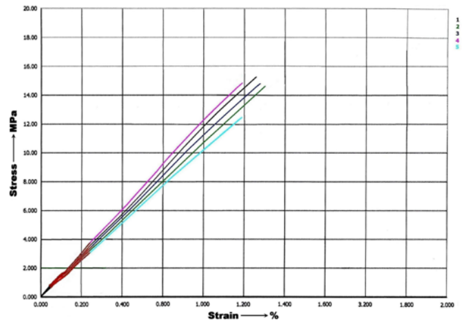
Figure 5. Stress-strain curve of pure polyester
