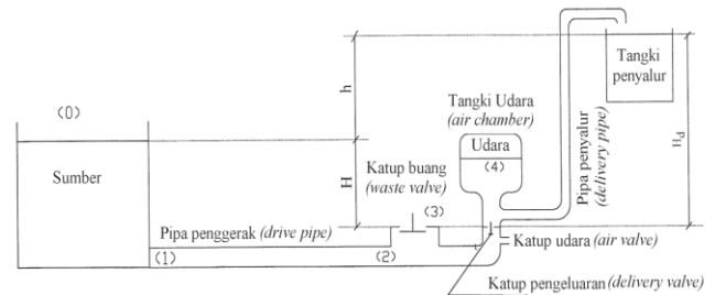
Gambar 3. Instalasi pompa hydraulic ram pump .
